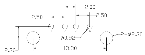
Recommended P.C.B Layout (±0.05) TOP
