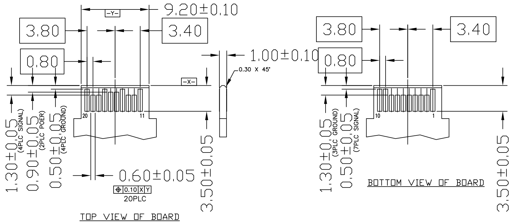
RECOMMENDED LAYOUT DETAIL MATING TRANSCEIVER PCB
