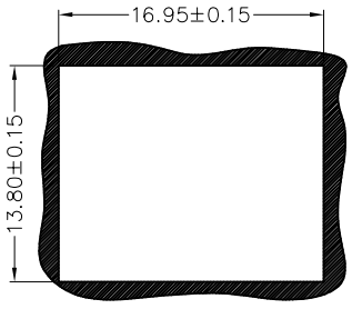
RECOMMENDED PANEL CUT
